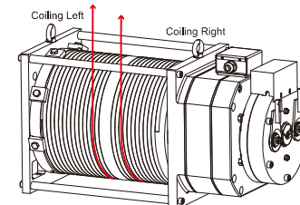
Bottom Installation, ropes out upward
