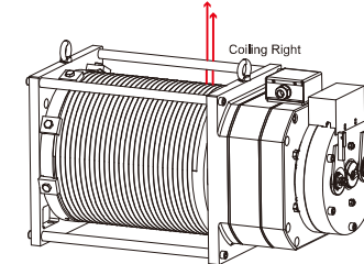
Bottom Installation, ropes out upward
